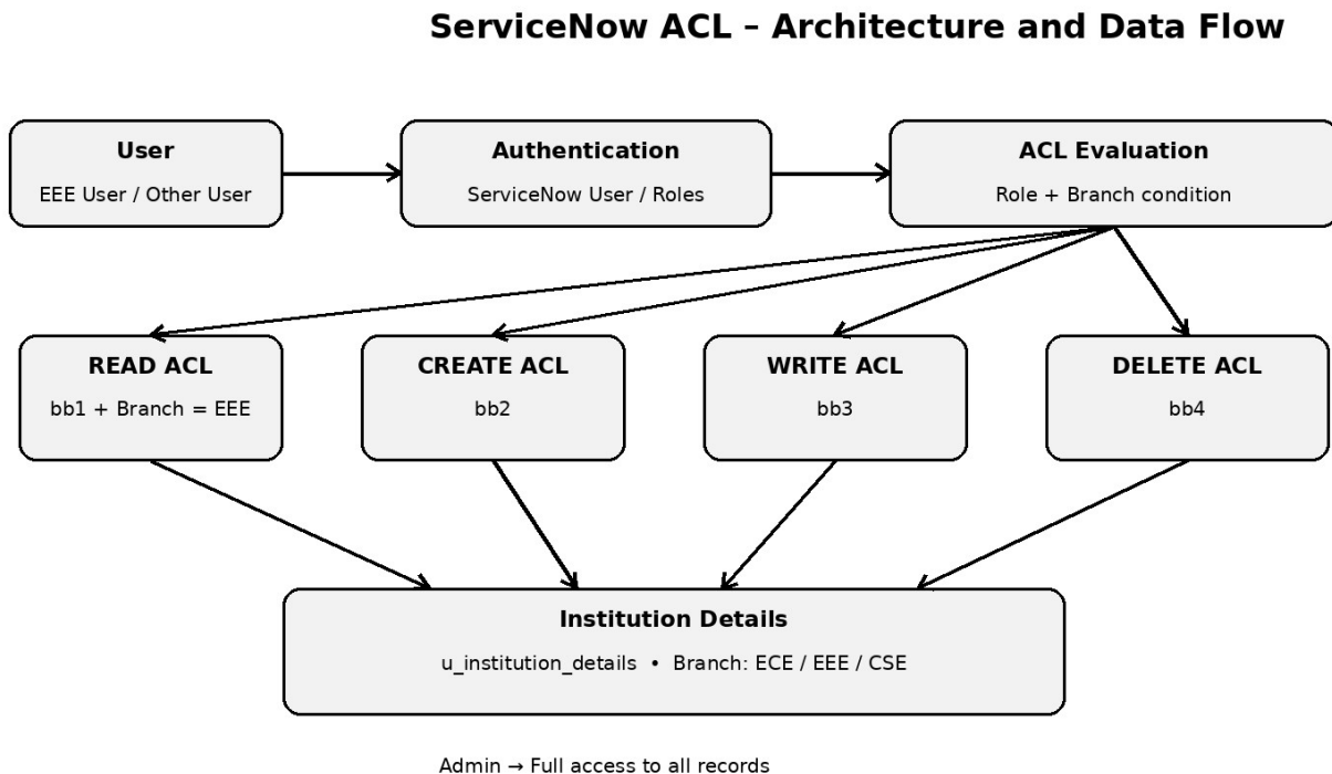
Figure 1: Architecture and data flow of the Script-Controlled ACL ServiceNow application
